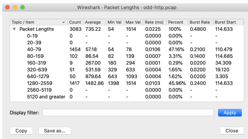
Figure 83. The “Packet Lengths” window
